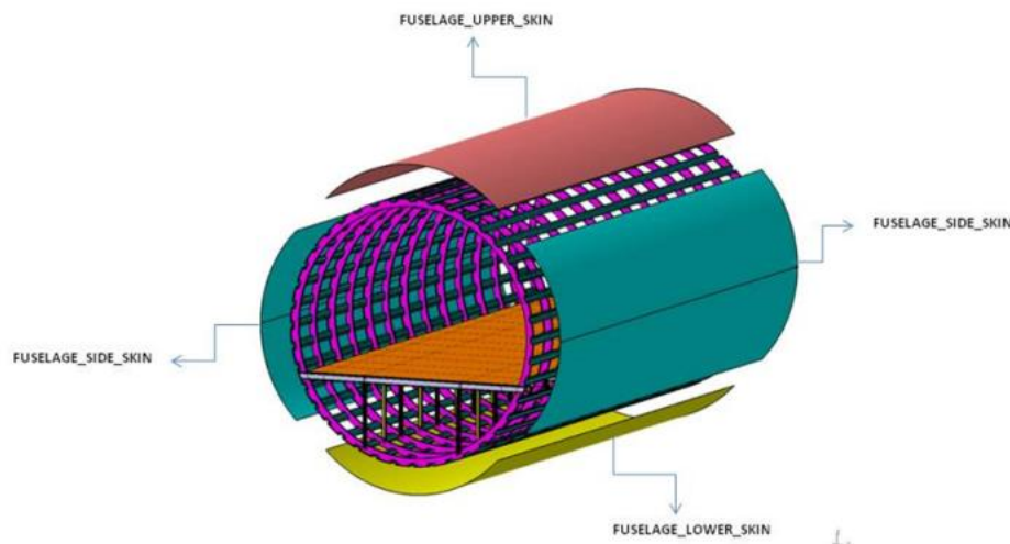
Figure 10: Fuselage components
