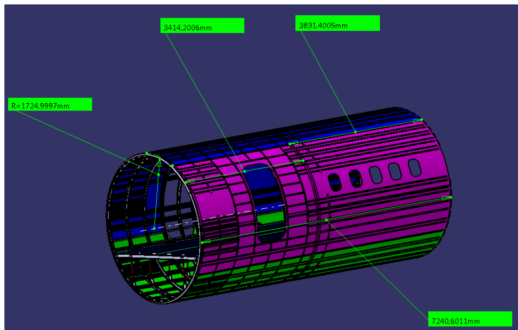
Fig. 4: General dimensions
