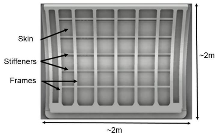
Figure 1: A typical structural configuration and size for an aircraft cargo door.
