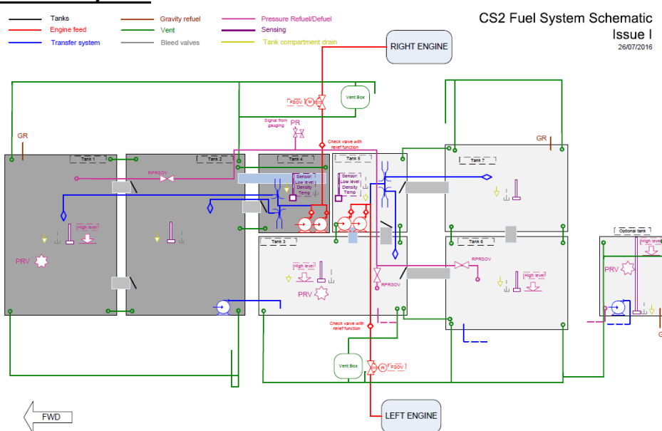
Schematic of the Fuel System
