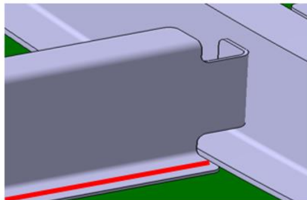
Figure 4: Schematic of a typical Z-profile stiffener welded against the skin. The weld is shown in red in the picture. Note that the position of FSSW would be in regular intervals along this line
