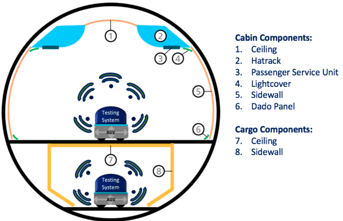
Figure 1. Cabin and Cargo Assembly Environment
